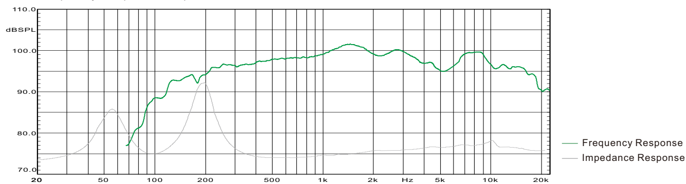
Frequency Response&Impedance
