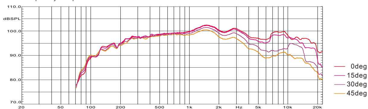
Frequency Response in Horizontal
